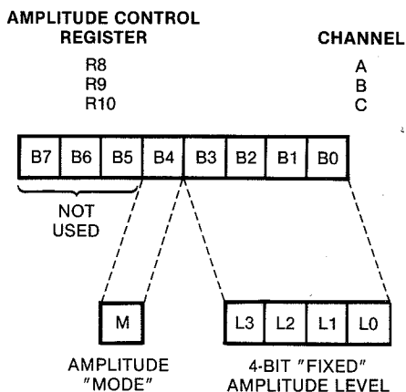
Fig. 7-7. Amplitude Control Registers. (Courtesy General Instrument Corp.)
